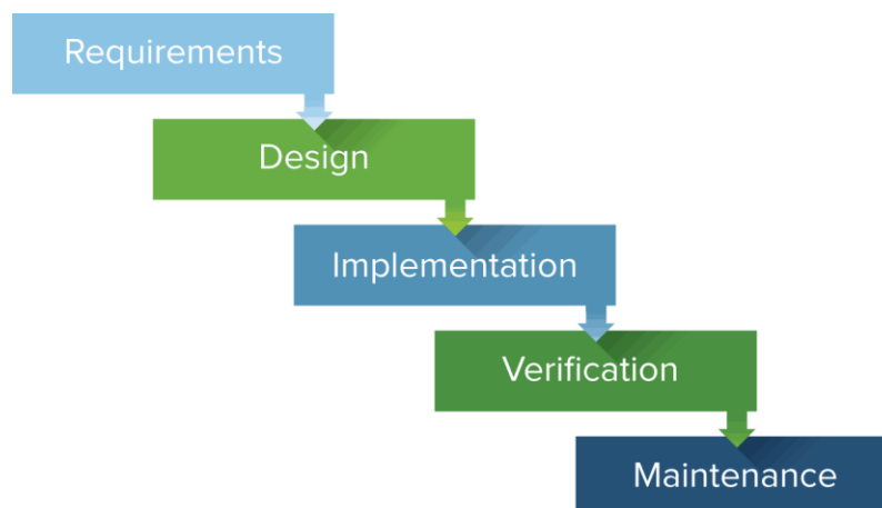
Gambar 1. Metode Waterfall
